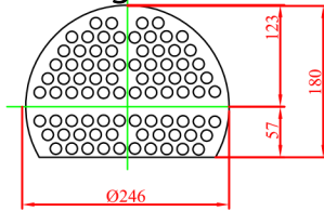
Segment pregrade \delta=3\text{mm}
